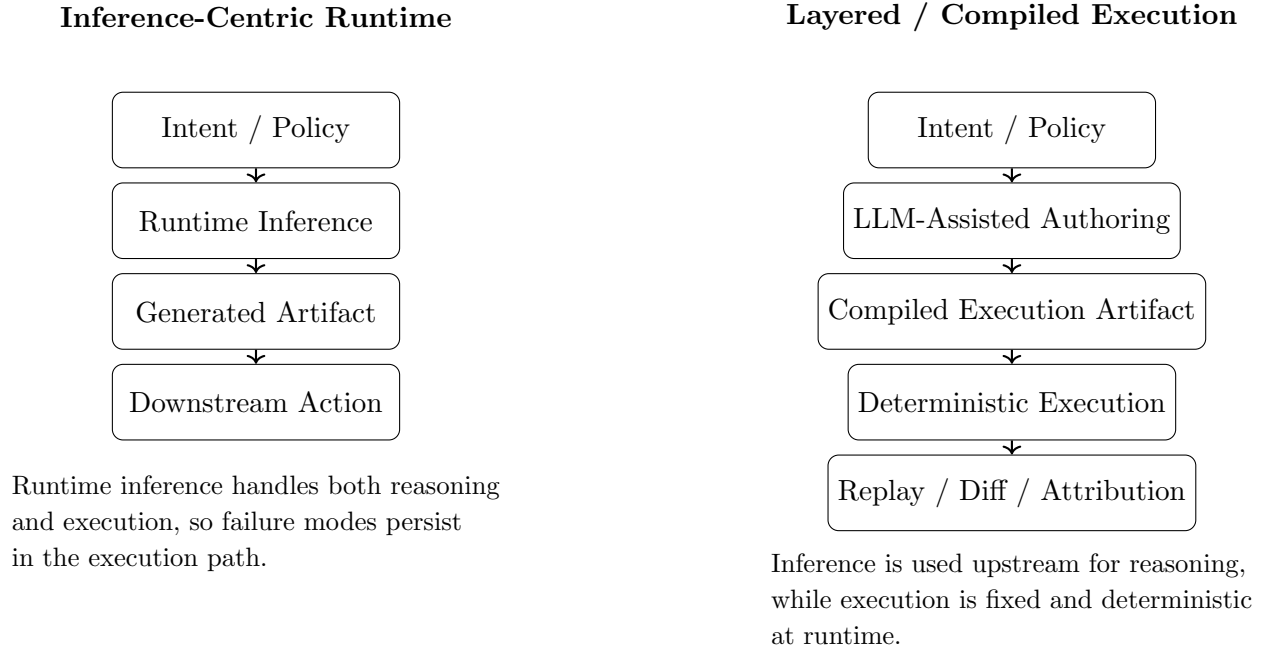
Figure 1: Two ways to position language models in an operational system. On the left, inference remains in the runtime execution path. On the right, inference is used upstream, while execution is performed through a compiled representation with fixed runtime behavior.
